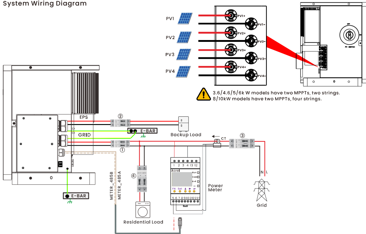
System Wiring Diagram
