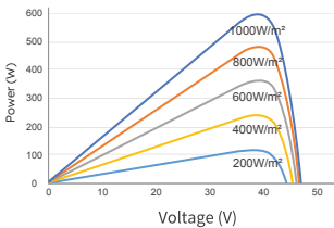
P-V Curves (595W)
