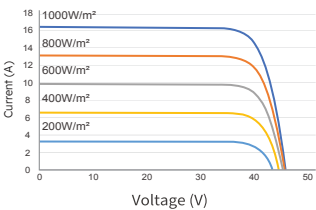
I-V Curves (595W)
